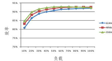
RSD-300D-24
