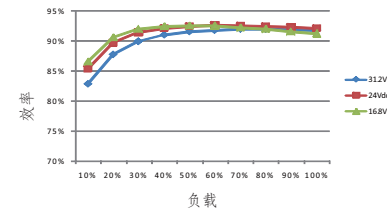
RSD-300C-24
