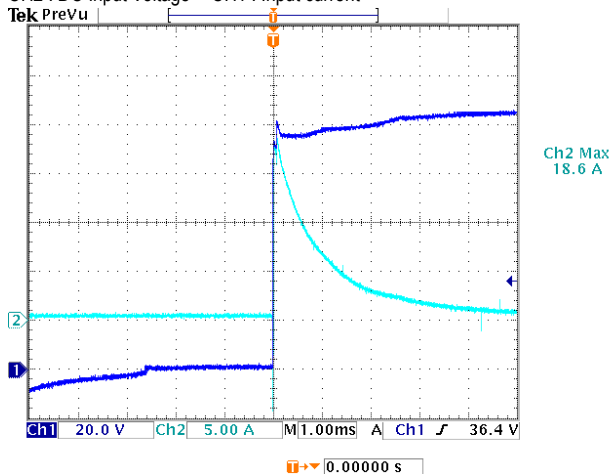
INPUT=110VDC @ FULL LOAD
