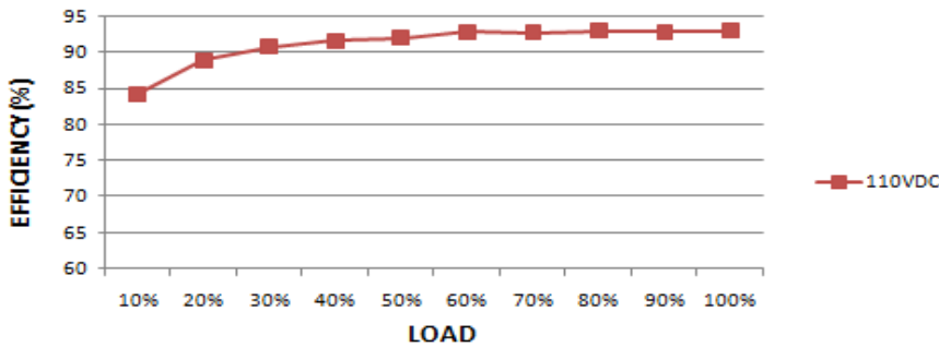
EFFICIENCY vs LOAD
